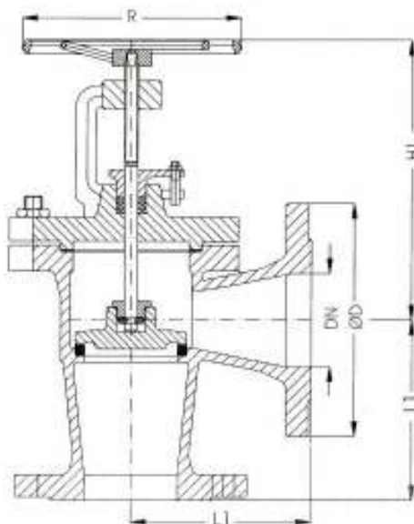
Type 018010 (Form B)
