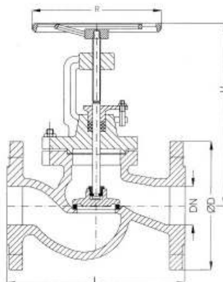
Type 017010 (Form A)
